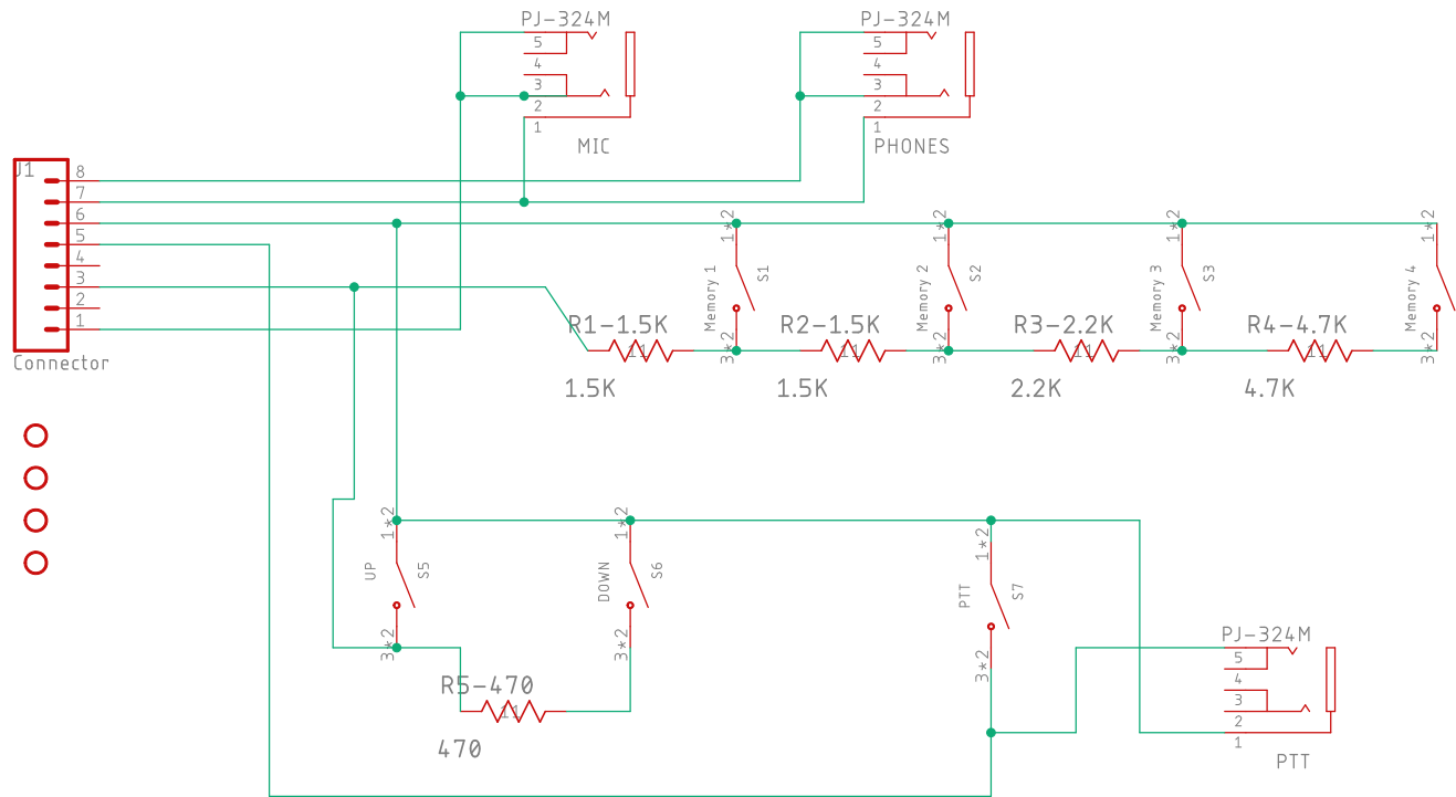
Icom External Keypad Project Version 1.00 by ON5IA
